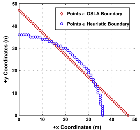
Fig. 10. Boundary of the optimal placement set (OSLA boundary) and boundary derived from the heuristic policy ( p = 0.002 , q = 0.5 and \eta = 2 ).
